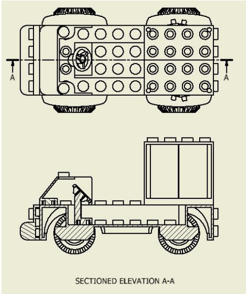
Sectioned Elevation
